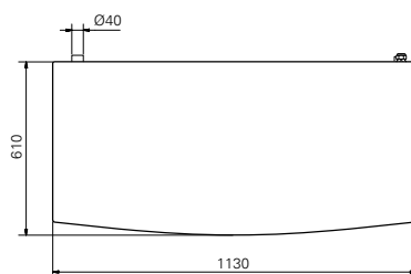
NIBE F2120-8
