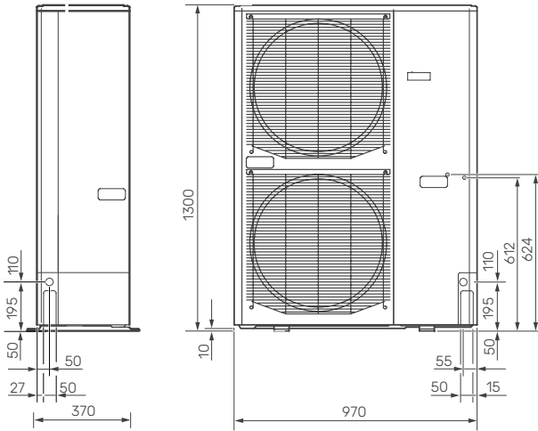
NIBE AMS 10-16
