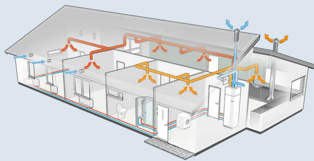
NIBE F470
