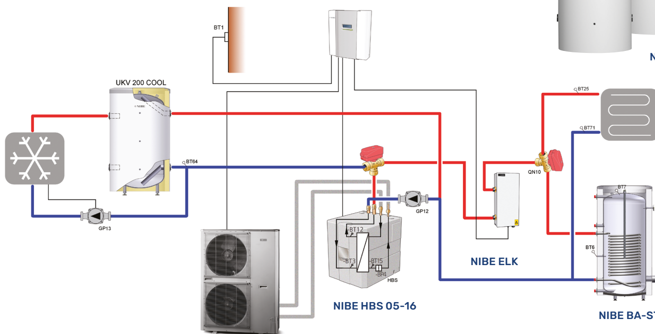
NIBE AMS 10-16
